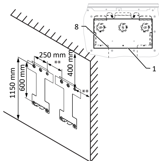
Abb. 12: Wandmontage
