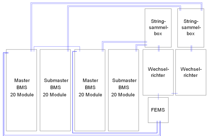
COK102 – 100 kW/420 kWh
