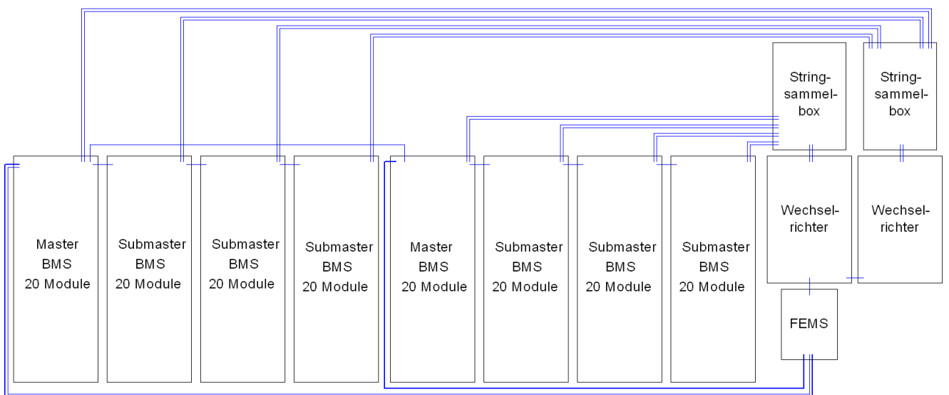
COK103 – 100 kW/560 kWh
