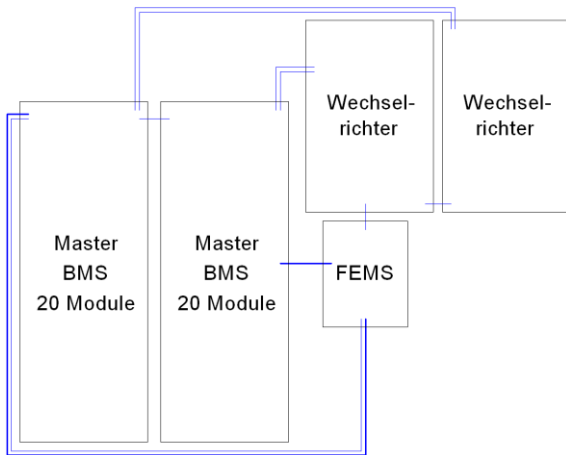
COK100 – 100 kW/140 kWh
