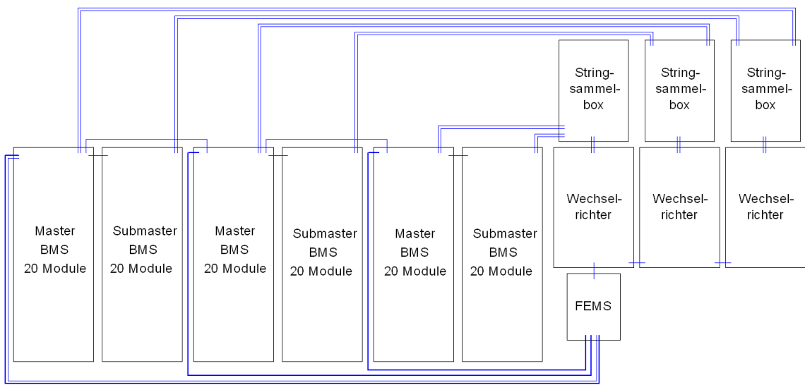
COK201 – 150 kW/420 kWh
